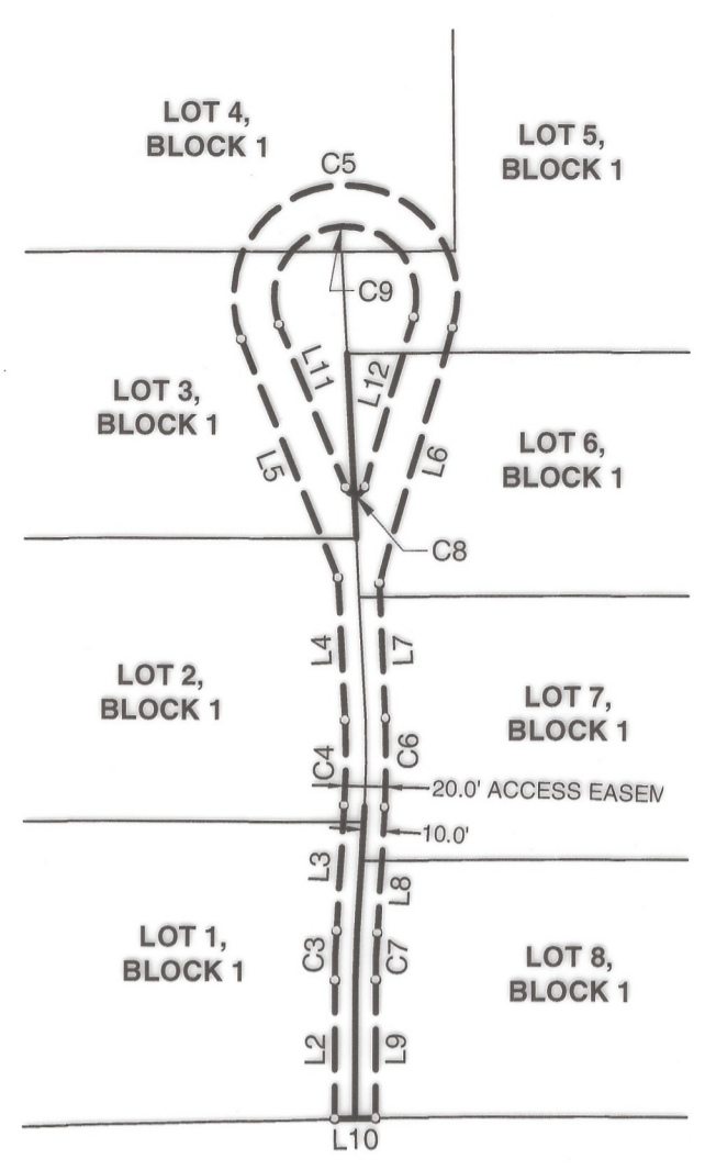
HOOVER LANE ACCESS AND UTILITY EASEMENT DETAIL SCALE: 1" = 100'
